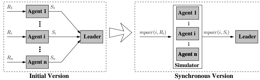
Fig. 1. Transformation to a Synchronous Protocol
